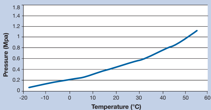
Vapor Pressure vs. Temperature – Metric Units
