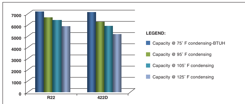
Performance characteristics of R-422D relative to R-22 at standard A/C conditions.
