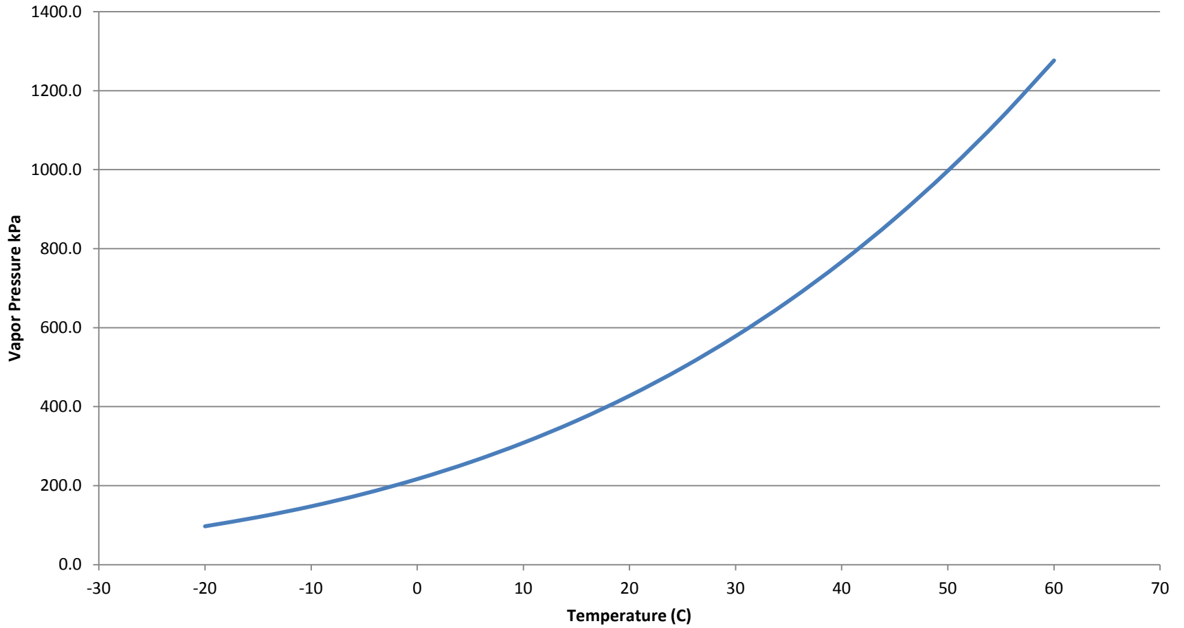
1234ze Vapor Pressure versus Temperature
