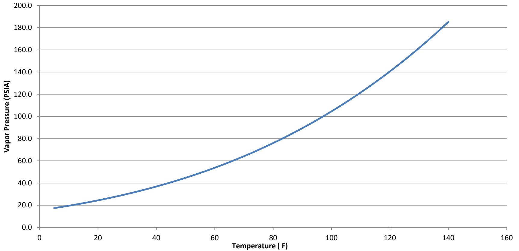
1234ze Vapor Pressure versus Temperature
